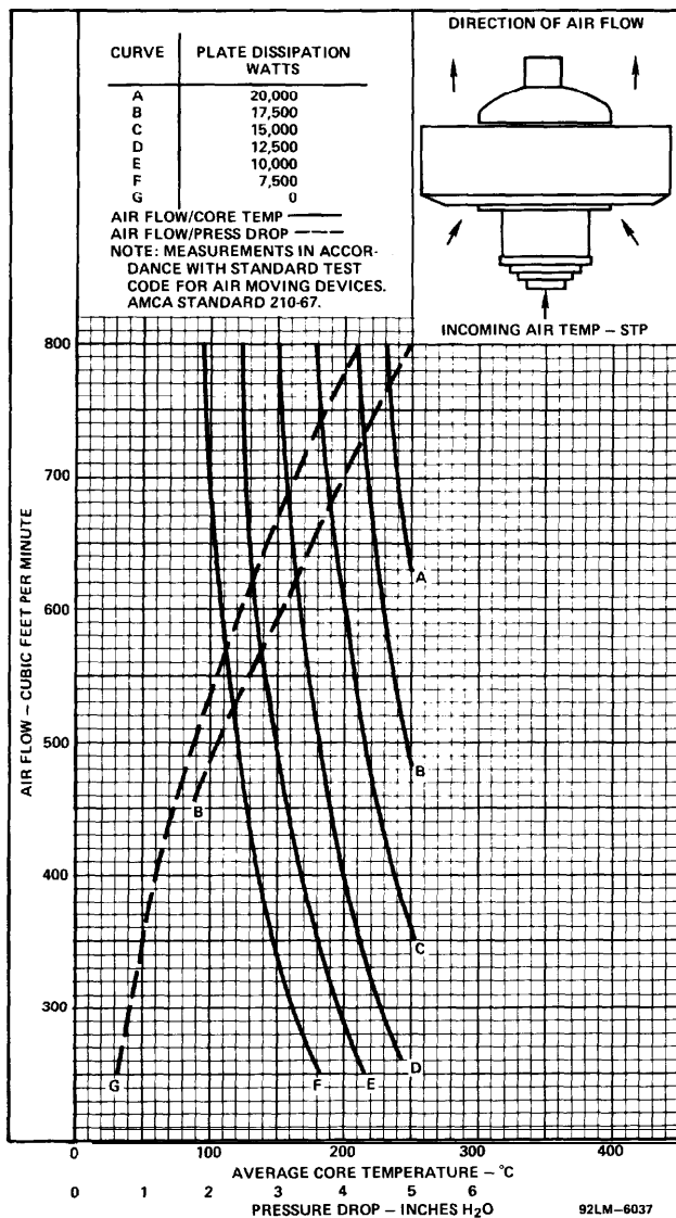
Figure 5 - Air Flow Characteristics
